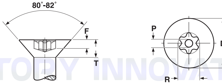
SIX-LOBE PIN-IN FLAT HEAD SECURITY SCREWS
