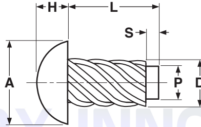
DRIVE SCREWS - ROUND HEAD TYPE U
