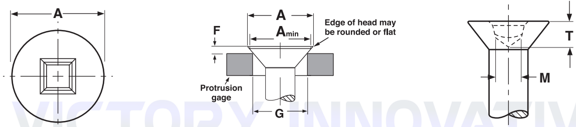
SQUARE RECESS FLAT HEADS
