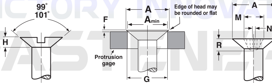
FLAT HEAD 100° FOR SELF-TAPPING SCREWS
