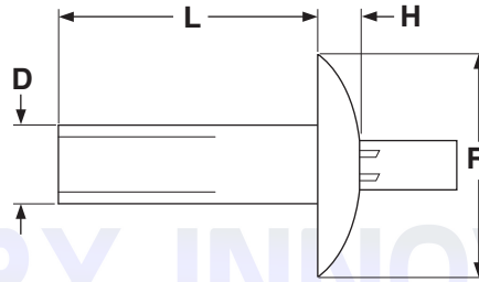
BRAZIER HEAD DRIVE PIN RIVETS
