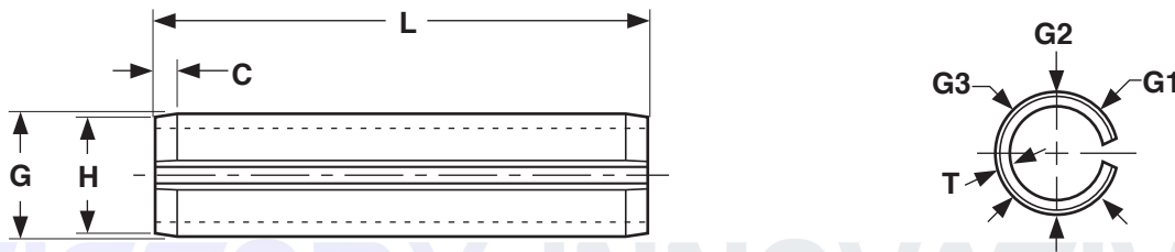
SPRING PINS, SLOTTED TYPE
